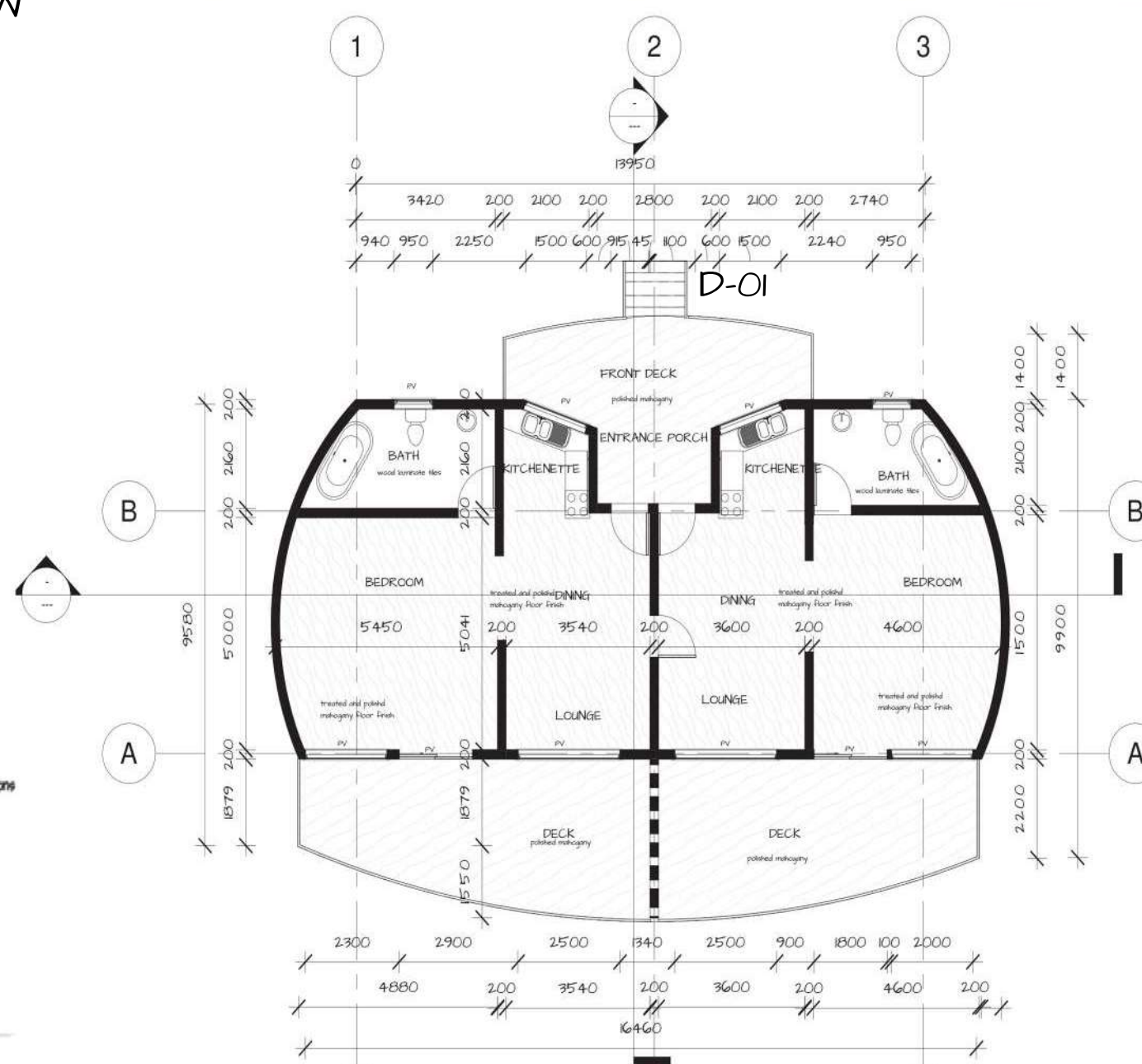
WORKING DRAWING 2 FLOOR PLAN 3
