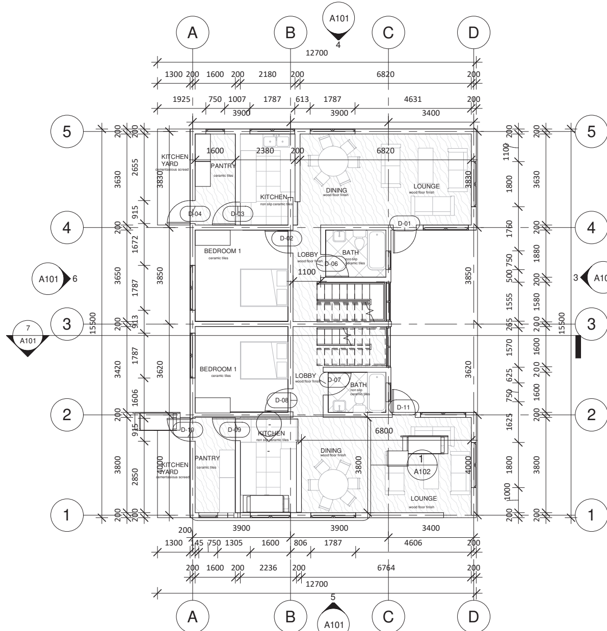
SEMI-DETACHED MAISONETTE FIRST FLOOR SCALE 1:100
