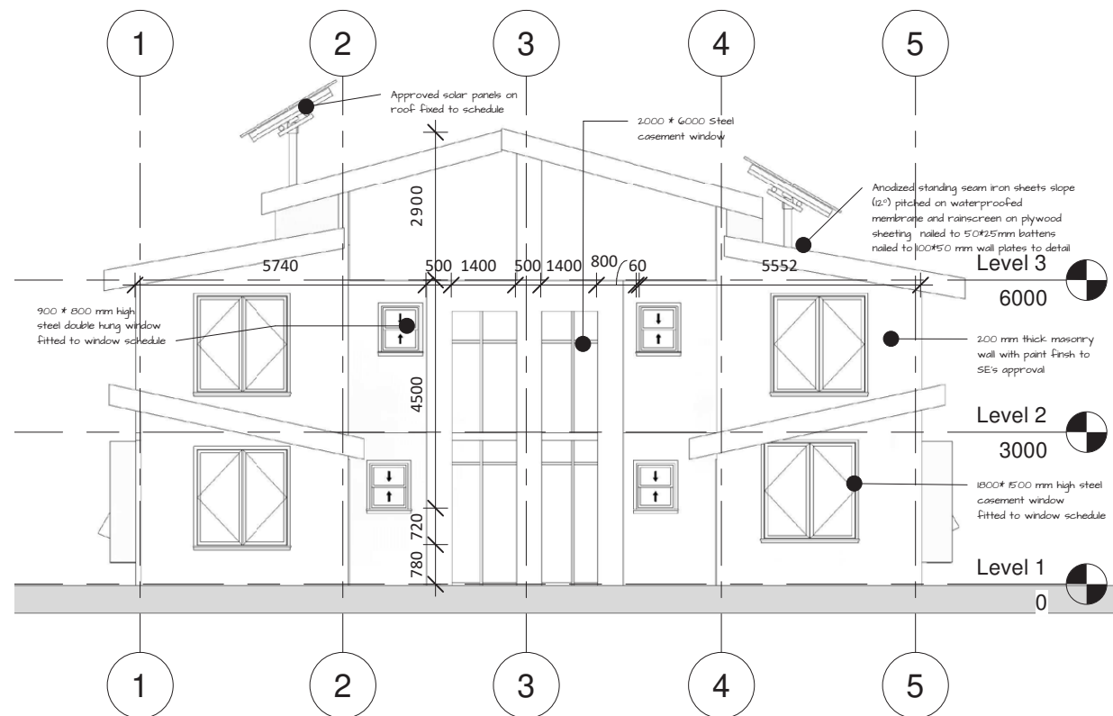
SEMI-DETACHED MAISONETTE FRONT ELEVATION SCALE 1:100
