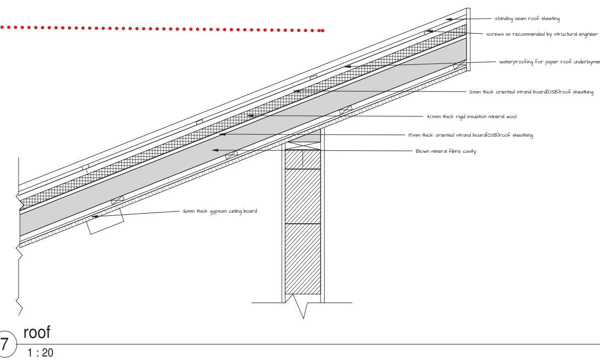
ROOF DETAIL
