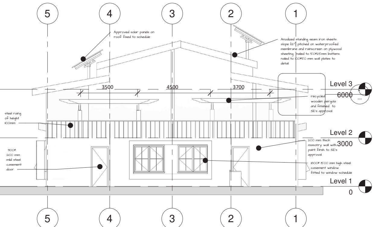
SEMI-DETACHED MAISONETTE BACK ELEVATION SCALE 1:100
