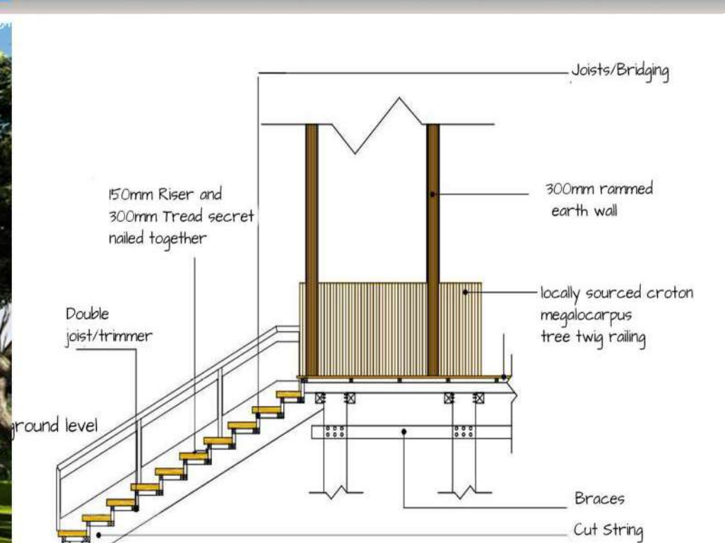
D-01 -OPEN RISER TIMBER STAIRS DETAIL
