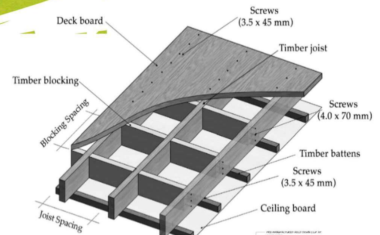
WOODEN FLOOR CONNECTION DETAIL
