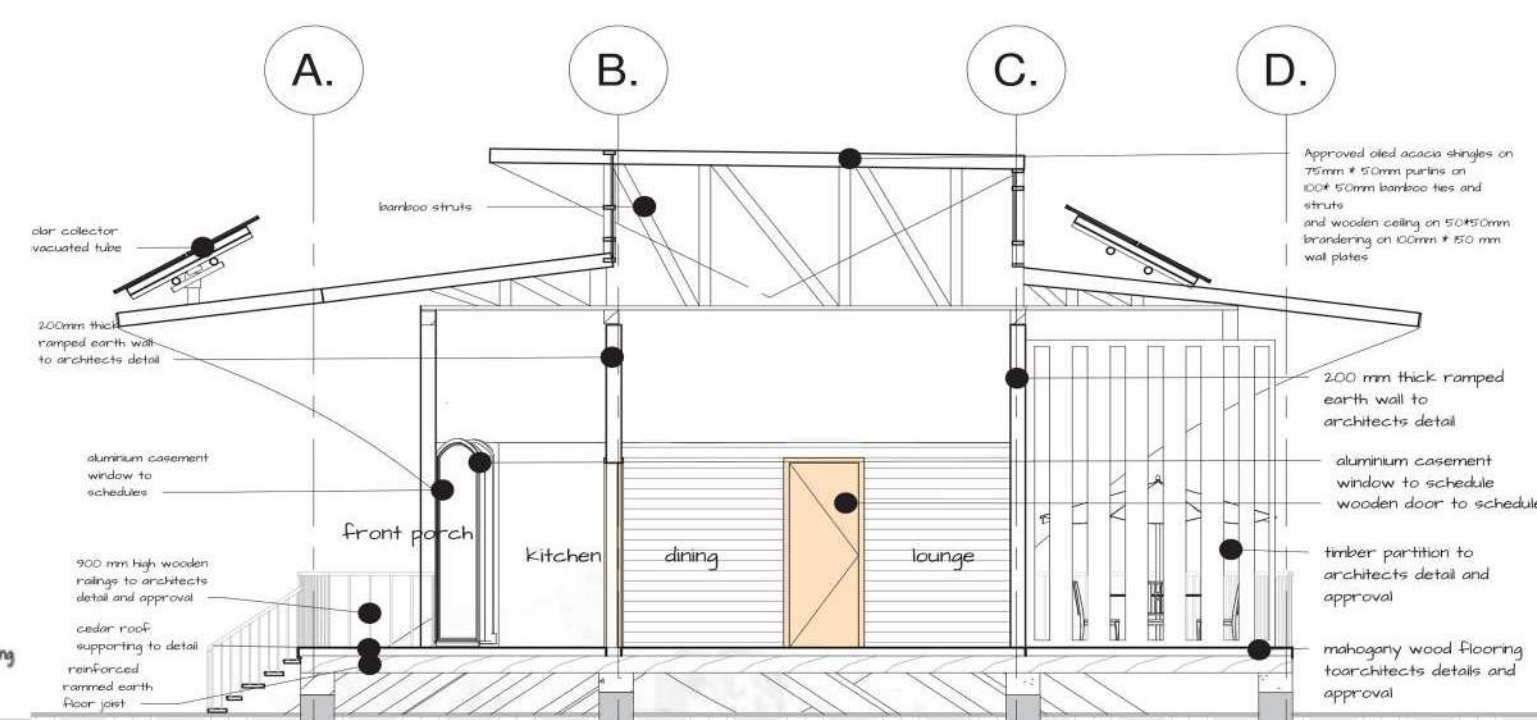
SECTION-01
